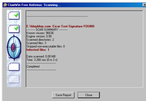
Antivirusprogramma ClamWin
